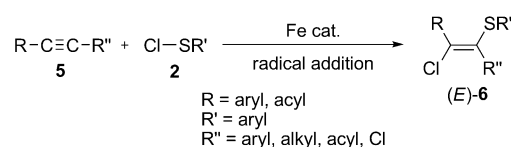
Scheme 1. Chlorothiolation of alkynes.
