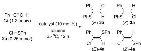
Scheme 2. Addition of benzenesulfonyl chloride ( 2a ) to phenylacetylene ( 1a ).
